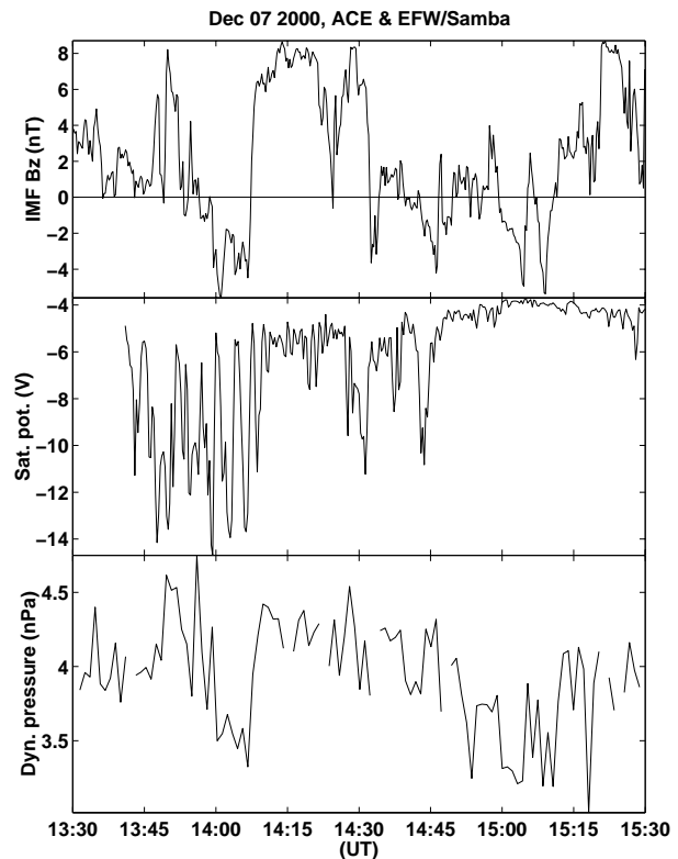
Fig. 8. (top panel) IMF B_z as recorded by ACE (time shifted with 80 min), (middle panel) negative of the satellite potential of Samba (s/c 3), and (bottom panel) dynamic pressure based on ACE/SWEPAM proton density and speed data.
