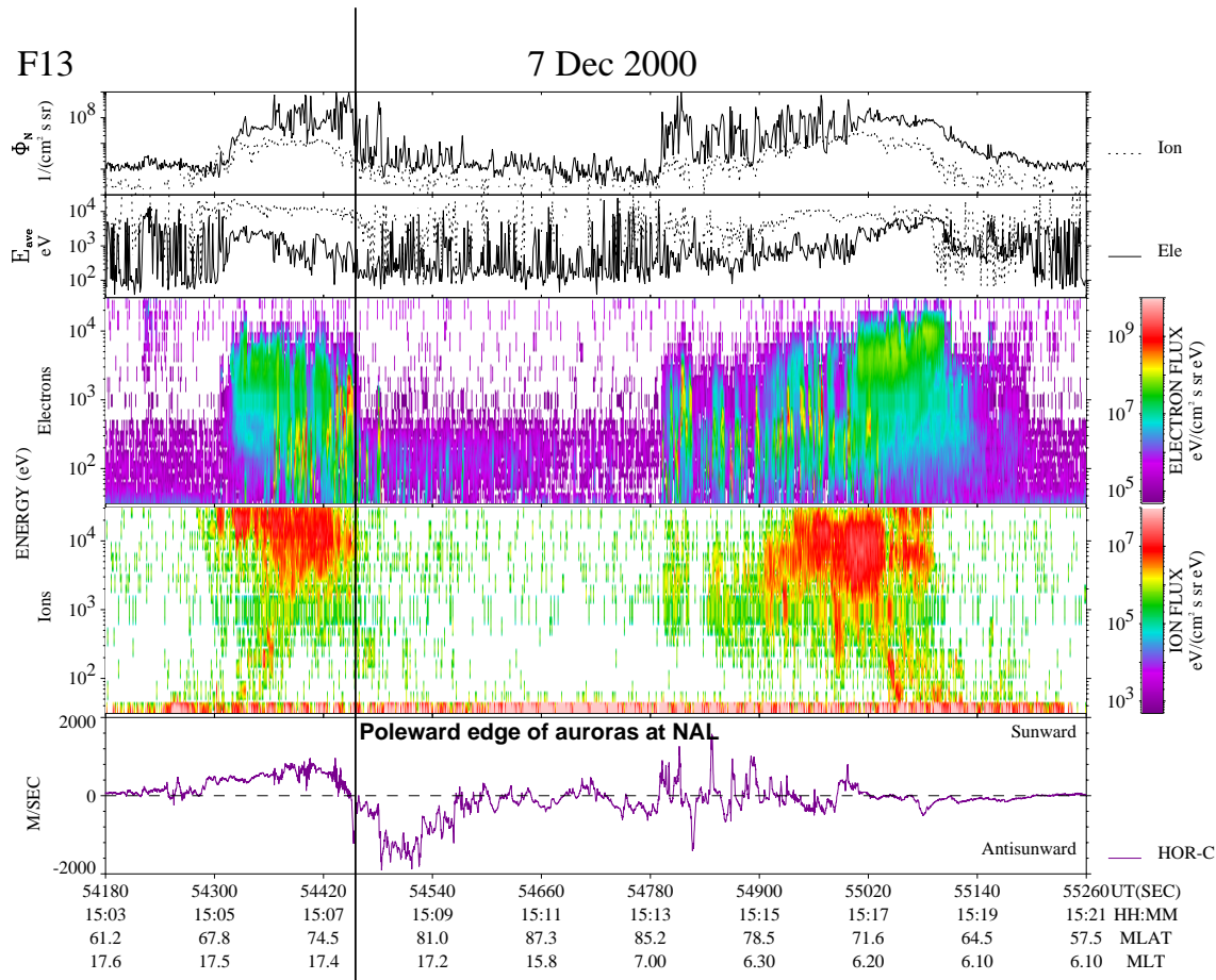
Fig. 6. Data recorded by DMSP F13 instruments during the track shown in Figure 5 (from top to bottom): Ion and electron number fluxes and average energies, spectra showing differential energy fluxes, and plasma flow velocities. The vertical line marks the location of the poleward edge of the auroras shown in Figure 5.
