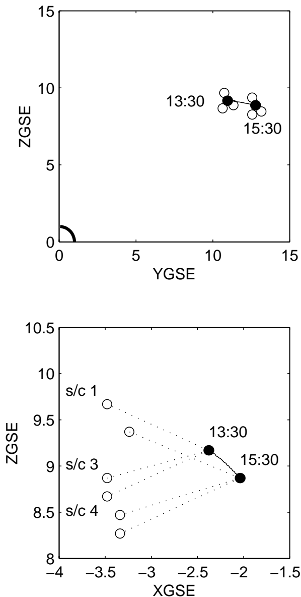
Fig. 7. Cluster orbit and configuration during 1330-1530 UT December 7, 2000 in GSE YZ and XZ planes. The solid line and black dots show the location of s/c 2 (Salsa). In the bottom panel the dashed lines join Salsa with the other spacecraft. For clarity reasons the real inter-spacecraft distances have been multiplied by 10.
