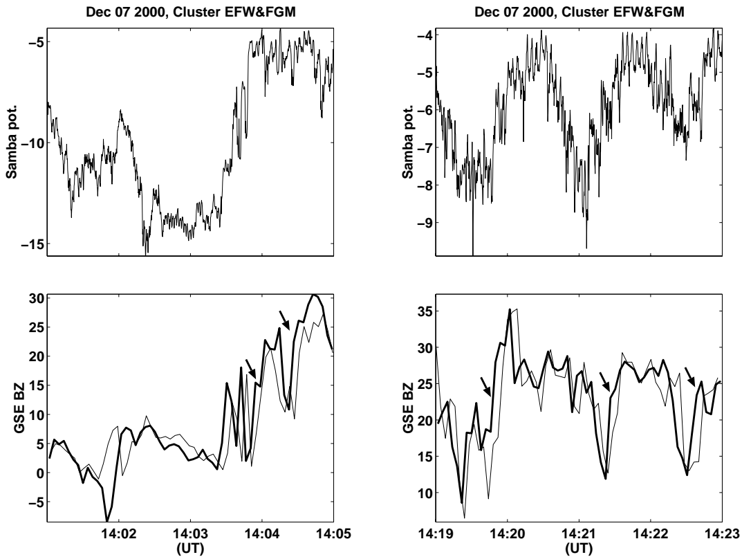
Fig. 9. Negative of the satellite potential of Samba and B_z (GSE) as recorded by Salsa (thick line) and Samba (thin line) FGMs. Left (right) panel shows an example recorded during the larger (smaller) potential variations. The arrows point the differences in the curves which have been used when estimating the phase velocities.
