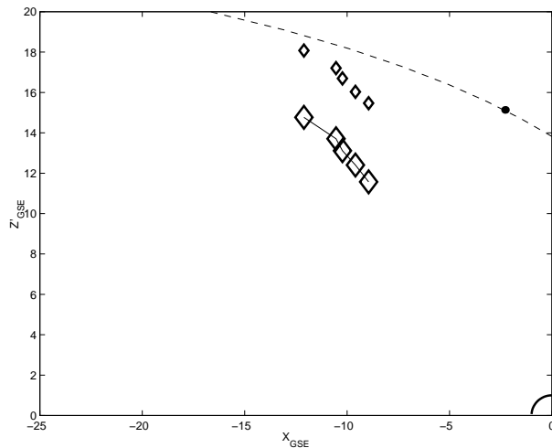
Fig. 10. The locations (the larger diamonds joined with the thin line) of the field lines conjugate with the poleward edge of auroras observed by ITACA at 14:46:20 UT (c.f. Figure 5) in the plane defined by the Samba location and the X-axis of the GSE coordinate system. The dashed line shows the magnetopause location according to the model by Shue et al. (1997). The smaller diamonds show the maximum radial extents ( R = (Y_{GSE}^2 + Z_{GSE}^2)^{1/2} ) of the traced field lines.
