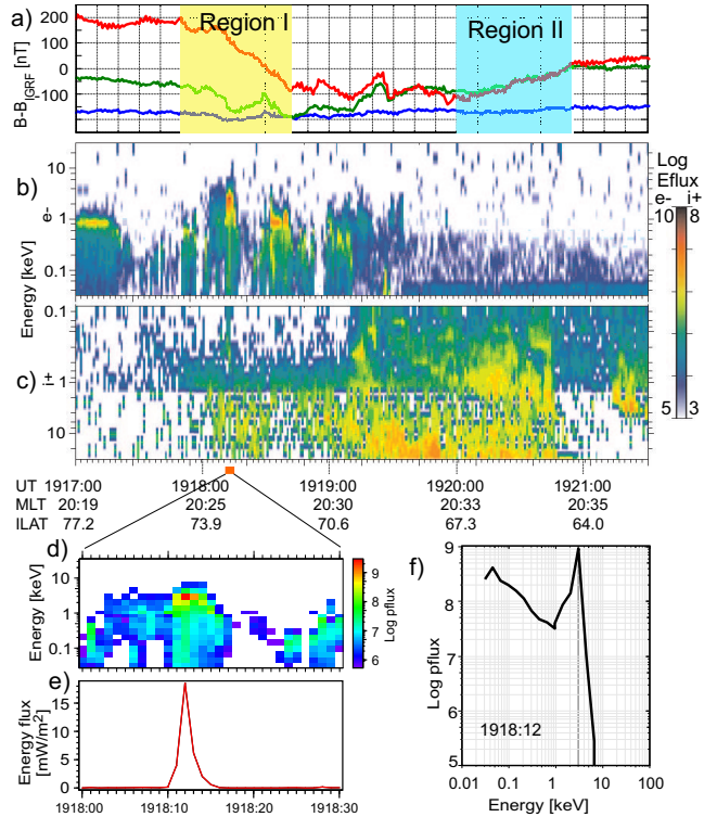
Figure 2. DMSP F14 observations. a) Magnetic field with IGRF model subtracted. Components are approximately: red eastward, green poleward, blue upward. b,c) electron and ion spectrograms. 30 s of data around the auroral arc, d) electron spectra and e) electron energy flux projected to ionosphere. f) electron number flux spectra from inside the inverted-V event.
