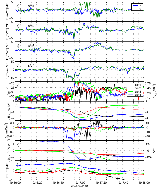
Figure 4. 2 min overview plot from all four s/c. The data have been low-pass filtered at 1 Hz. a–d) E in mean field coordinates, x is poleward and y is eastward. e) Probe to spacecraft potential and derived density estimate. f) integrated potential, the labels on the right show values if the arc motion is taken into account. g) Field-aligned Poynting flux calculated from total E and dB. h) integrated Poynting flux, it is set to zero at the beginning of the interval, marked by dots, that is used to estimate the total integrated energy flux. For g) and h) labels on the right show values at the ionosphere. i) Poleward component of dB in field aligned coordinates.
