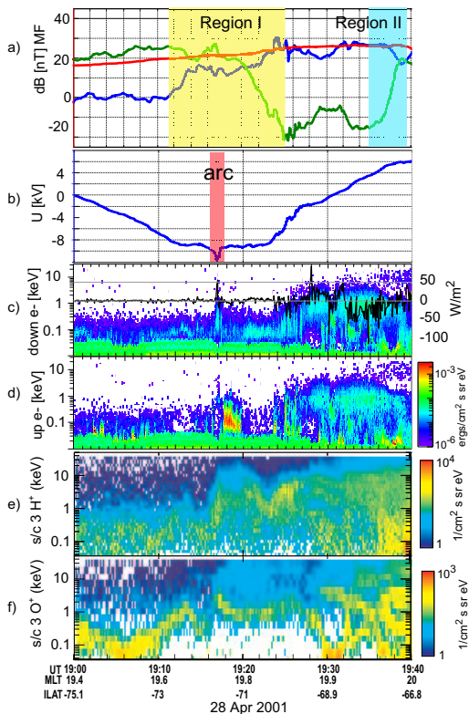
Figure 3. Overview plot of s/c 3 data. a) Magnetic field disturbance dB, subtracting the Tsyanenko 89 model, in field aligned coordinates. The approximate directions are — green eastward, blue poleward, red field-aligned. b) Potential integrating E along the satellite orbit. To obtain full E from EFW spin plane measurements we assume that E_{\parallel} = 0 . c,d) Spectrograms of electrons propagating parallel and antiparallel to B. c) line plot shows integrated electron energy flux, labels are on the right side. e,f) H + and O + spectrograms integrated over all pitch angles.
